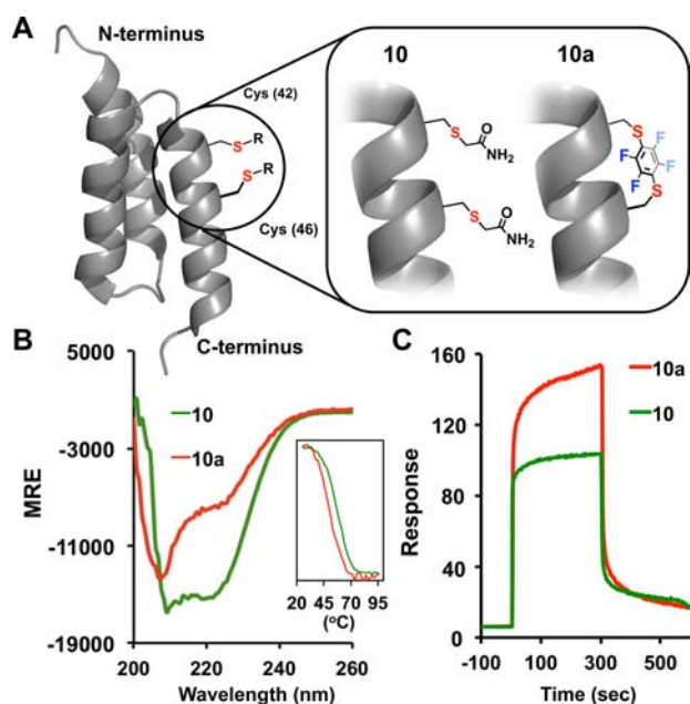
Figure 4. (A) Representation of the HER-2 affibodies (PDB code: 2B89) with chemically modified Cys positions [Cys 42 , Cys 46 ] via stapling (10a) and alkylation (10). (B) CD spectra of 10 and 10a, and the corresponding temperature-dependent melting curves measured from the CD spectra at 222 nm (inset). (C) Biacore binding sensograms of 10, 10a with immobilized HER-2 extracellular binding region (adsorption/desorption time, 300 s).
