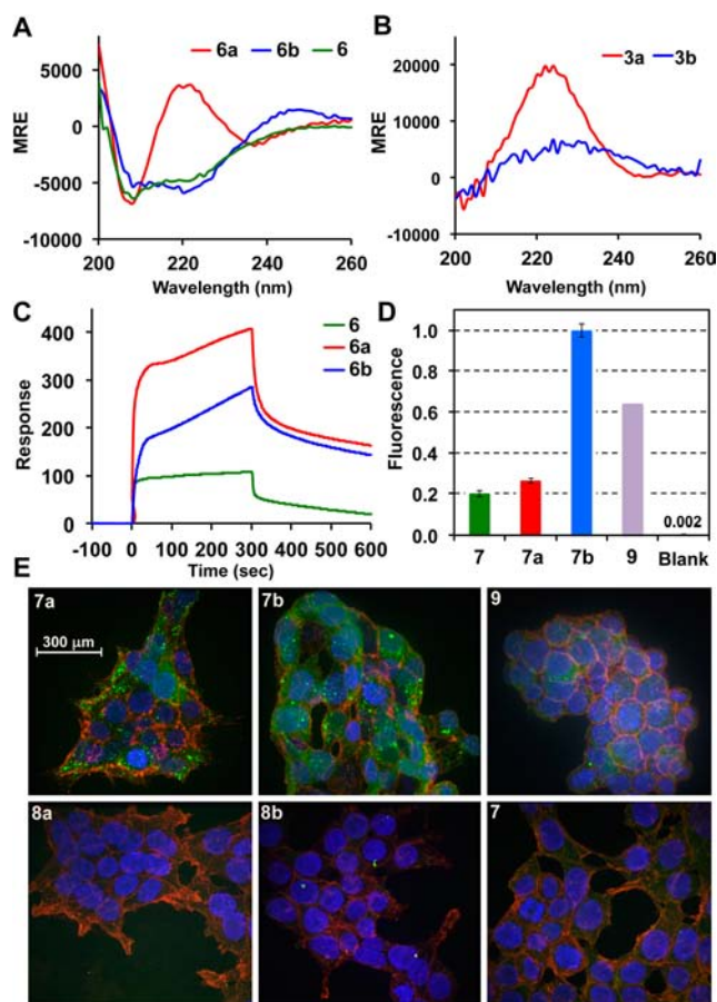
Figure 3. (A) CD spectra of 6 and 6a,b and (B) of 3a,b . (C) Biacore binding sensograms of 6 and 6a,b with immobilized C-CA (adsorption/desorption time, 300 s). (D) Flow cytometry data for FITC-based peptides incubated with HEK293T cells (25 \mu M; fluorescence response is averaged for each sample and normalized to 7b ). (E) Z-stack accumulated fluorescent confocal microscopy images (DNA, blue; cell membrane, red; peptides, green (FITC)) of the HEK293T cells treated with peptides 7 , 7a,b (5 \mu M), unstapled controls 8a and 8b and NYAD-2, 9 .
